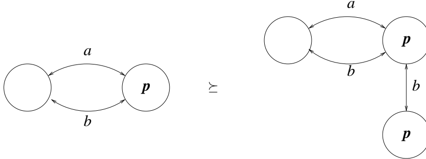
Fig. 1. The refinement in Example 3.7.
